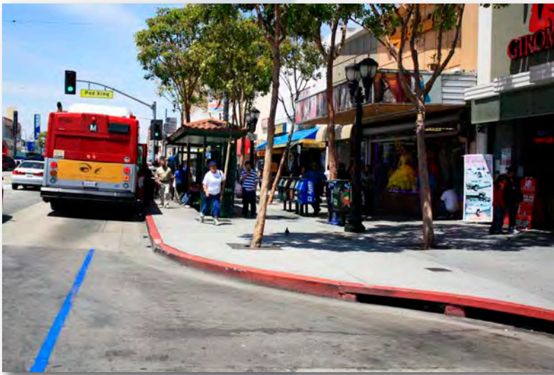
Bus bulbs: Huntington Park and Alhambra, CA (Credit: Sky Yim)
