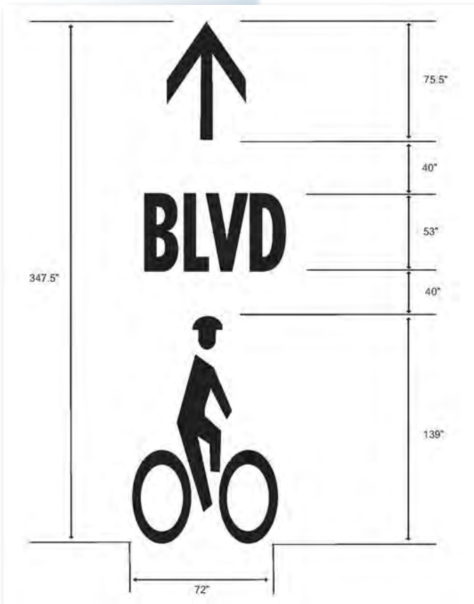
Bicycle boulevard pavement marking (Berkeley, CA)
