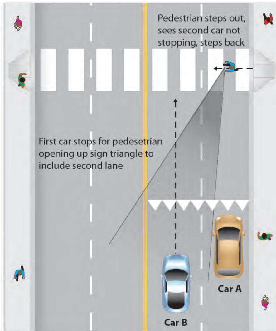
Advanced yield markings (Credit: Michele Weisbart)
