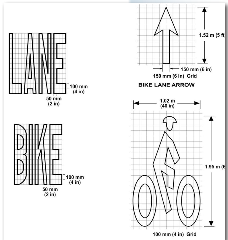
Bicycle lane markings (CA MUTCD Figure 9C-6)
