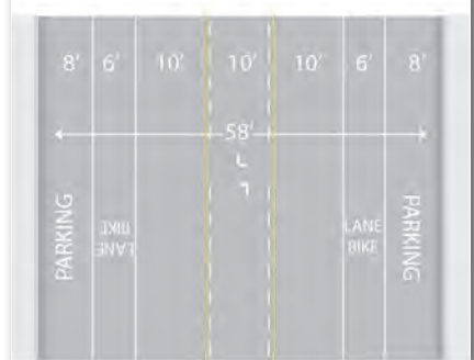
Fitting bicycle lanes with road diet (Credit: Michele Weisbart)
