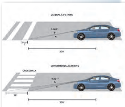
Longitudinal crosswalk markings are more visible than lateral crosswalk markings (Credit: Michele Weisbart)
