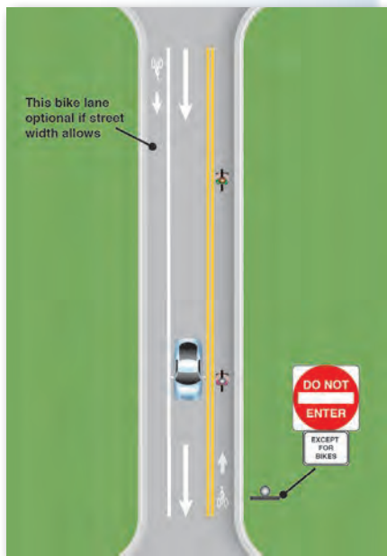
Contra-flow bicycle lane design (Credit: Michele Weisbart)
