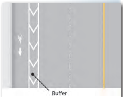
Painted-buffer bicycle lanes (Credit: Michele Weisbart)
