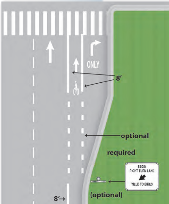
Bikeway markings at intersections (Credit: Michele Weisbart)
