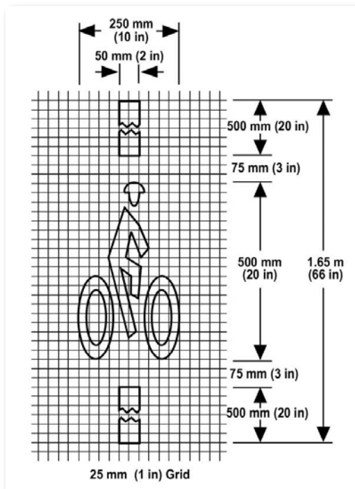
Bicycle detector symbol (CA MUTCD Figure 9C-7)
