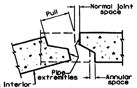
DETAIL A TYPICAL JOINT FOR REINFORCED CONCRETE PIPE
