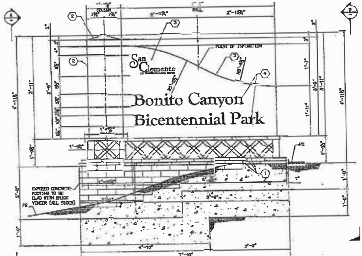
ENTRY MONUMENT SIGN - ELEVATION (EXPOSED FOOTING) SCALE 1" = 1'-0"
