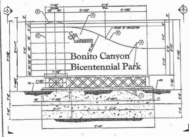
ENTRY MONUMENT SIGN - ELEVATION SCALE 1" = 1'-0"
