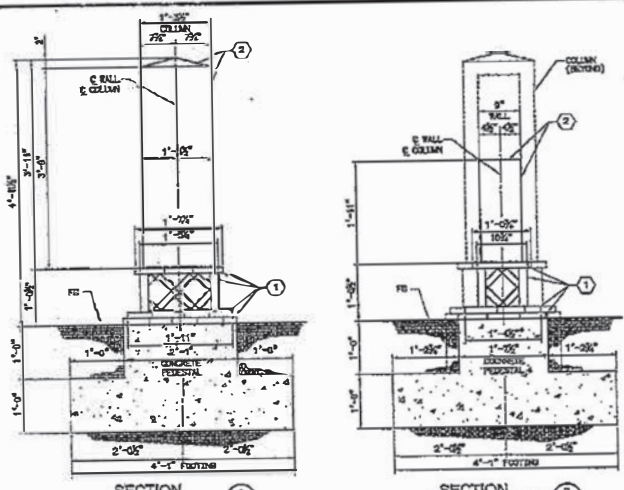
SECTION A-A SCALE 1" = 1'-0" SECTION B-B SCALE 1" = 1'-0"
