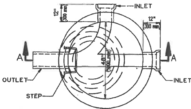
PLAN SHOWING BASE
