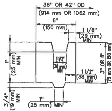
ADJUSTING RING DETAIL
