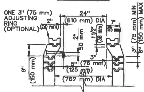
REDUCER RING AND ADJUSTING RINGS
