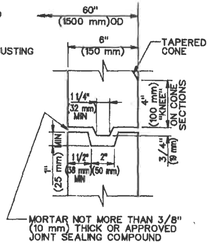
JOINT DETAIL NON-REINFORCED
