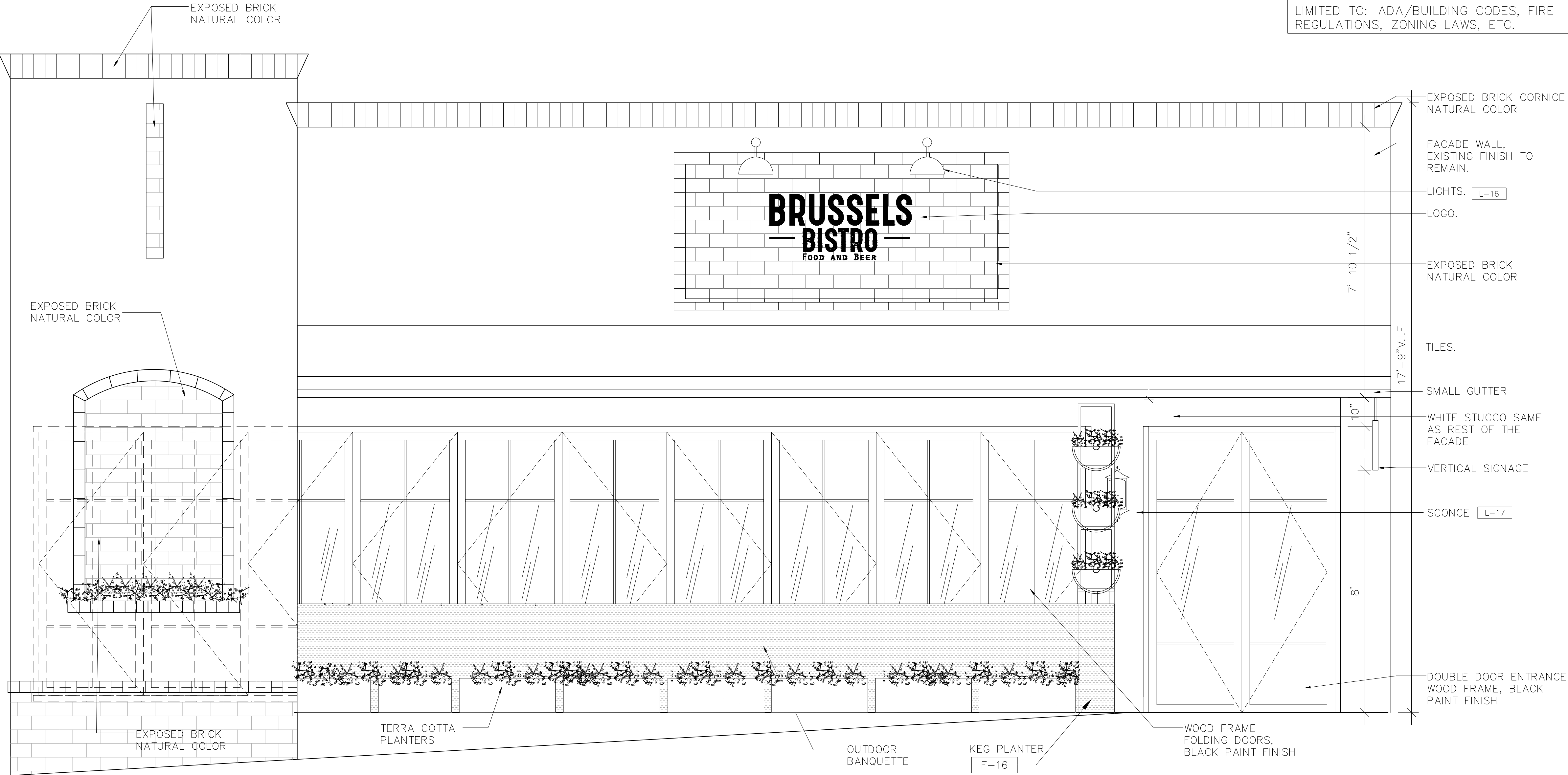
1 FACADE ELEVATION D6.0 SCALE: 3/4"=1'-0"
